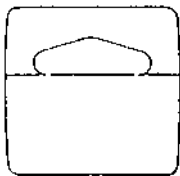
#4 Sen 1-5/8" wide x 1-3/8" high
